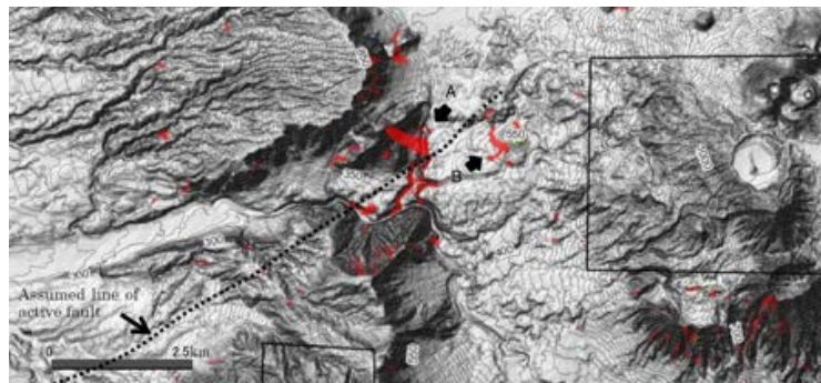
Fig.7 Preliminary analysis of landslides distribution and collapses in the west area of Voleano (Assumed fault line is added.) Prof. Chigira and Matsushi, Disaster Prevention Research Institute, Kyoto University
