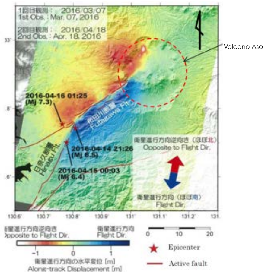
Fig.5 MAI (Multiple Aperture Interferometry) analysis using ALOS-2/PALSAR-2 Geospatial Information Authority of Japan (GSI) http://www.gsi.go.jp/cais/
