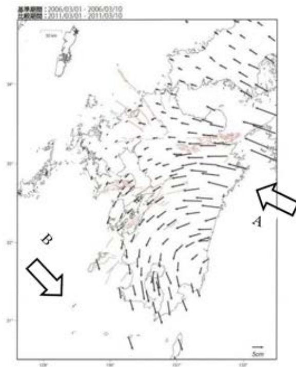
Fig.3 Average speed vector of displacement in the 5 years since March 2006 A: Compressive stress caused by Philippping Plate B: Expanding of Okinawa Trough
