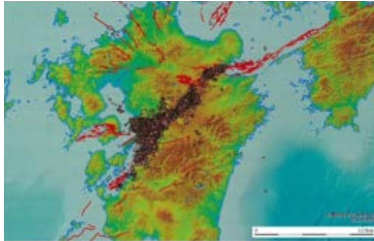
Fig.4 Distribution of the epicenters since April 14 2016 (At May10, 14:46) National Research Institute for Earth Science and Disaster Resilience (NIED) Disaster Information Laboratory http://www.bosai.go.jp/
