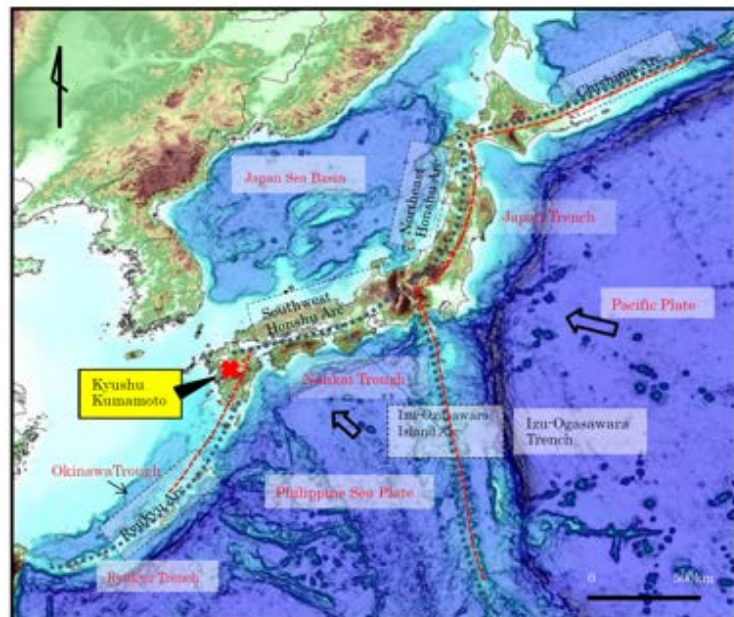
Fig. 1 General topographic view around Japan
