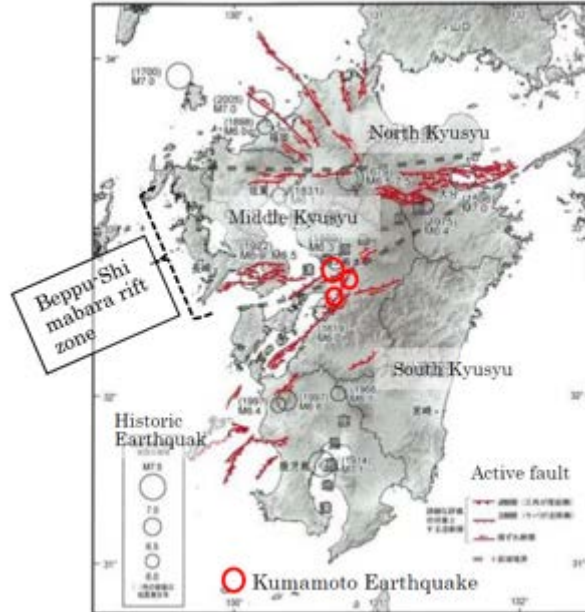
Fig.2 Active faults and historic Earthquake in kyushu
